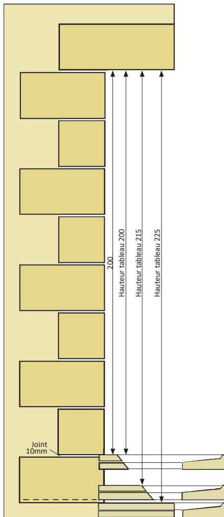
Jambage 200-225
